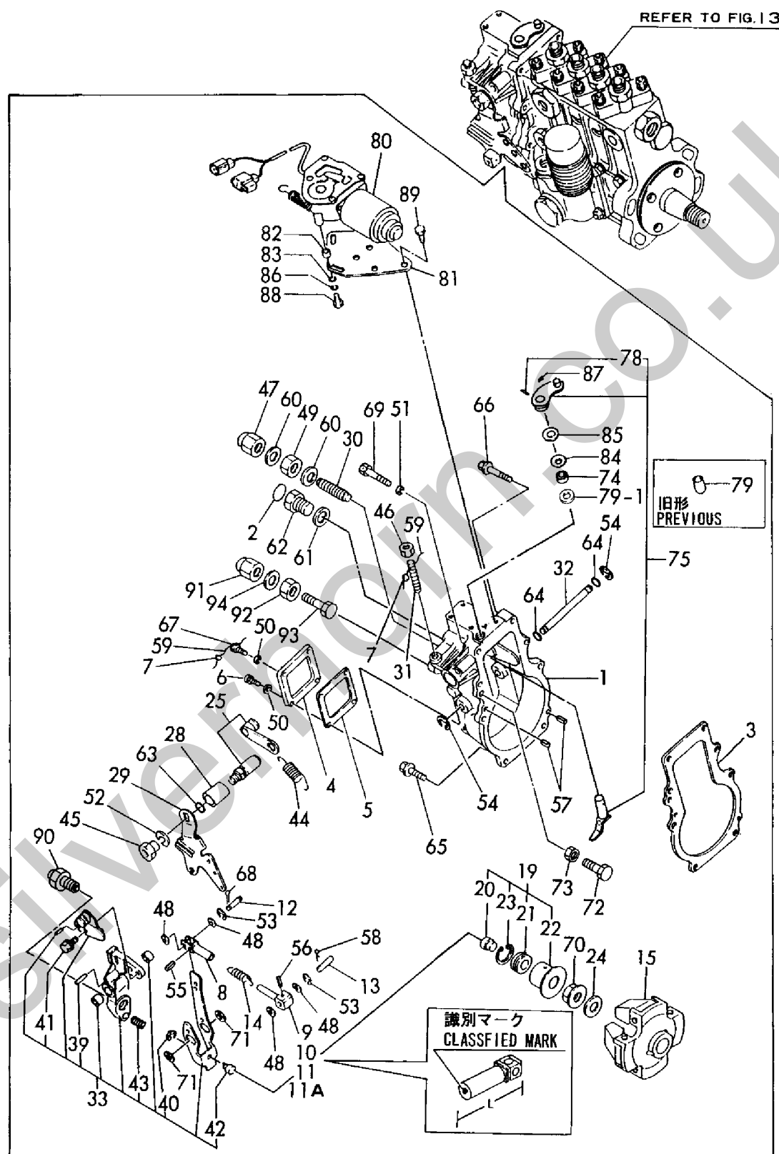
Fig. 14 ガバナ GOVERNOR
